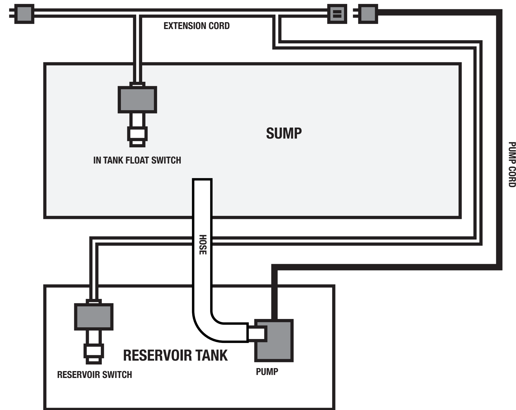
WIRE SCHEMATIC FOR ATO SYSTEM WITH 2 FLOAT SWITCHES
