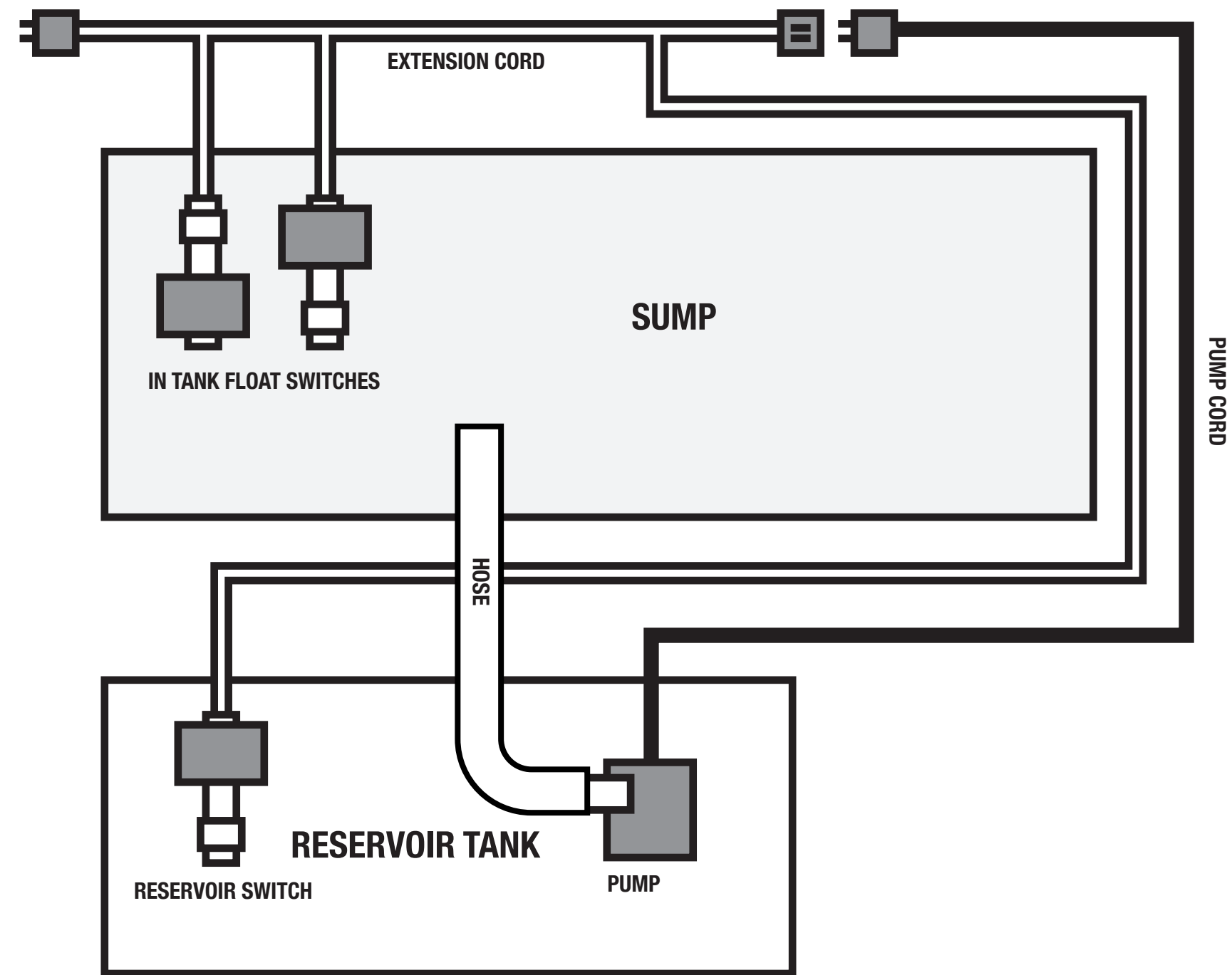
WIRE SCHEMATIC FOR ATO SYSTEM WITH 3 FLOAT SWITCHES
