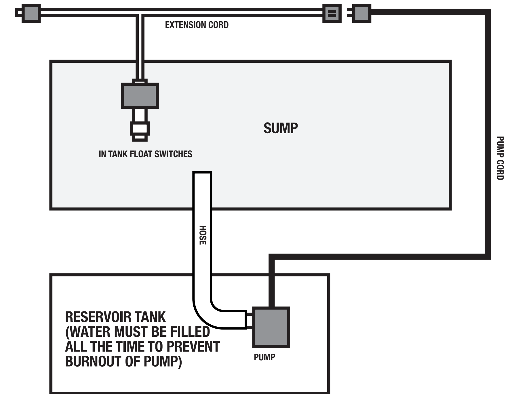
WIRE SCHEMATIC FOR ATO SYSTEM WITH 1 FLOAT SWITCH
