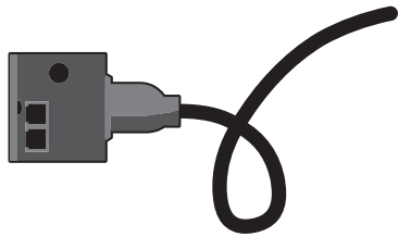
Correct Installation w/ Drip Loop
