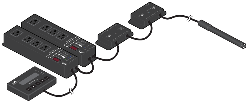
ReefKeeper Lite NET: Connection Example
